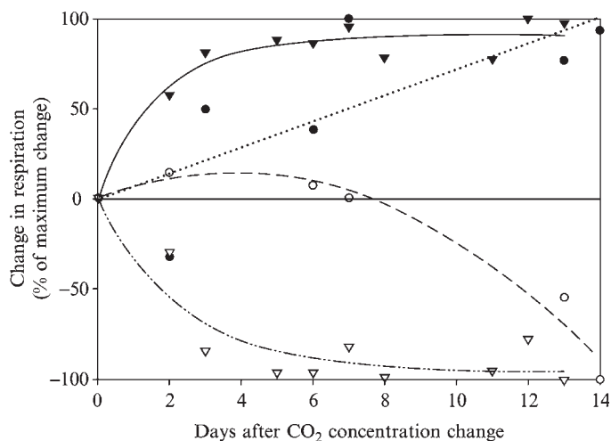
Figure 2: Effect of changing the atmospheric CO 2 conditions on ecosystem [(East bay }, (West bay II)] and soil [(East Bay -), (West Bay o)] respiration. Responses are expressed as a percentage of the maximum change occurring during the 2 week period.
